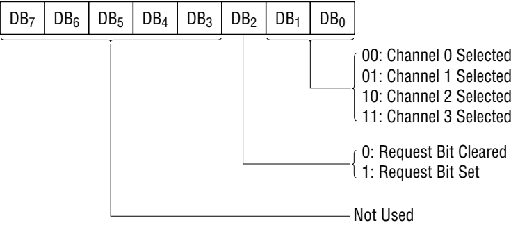
Figure 5 Request Register
