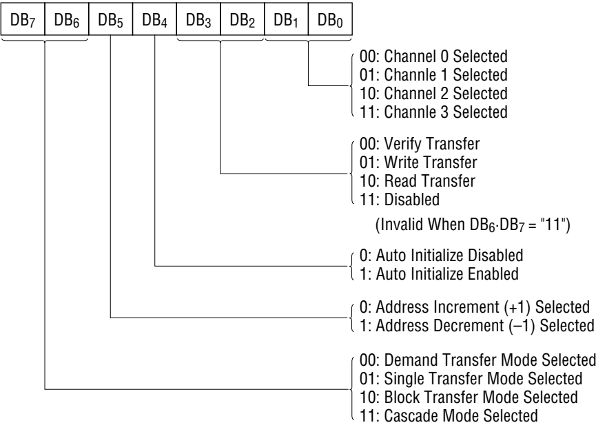
Figure 4 Mode Register
