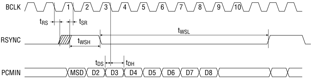
Figure 1 Basic Timing
