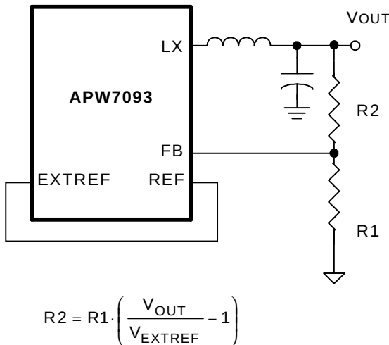
FIG.5 Adjusting the Output Voltage using FB
