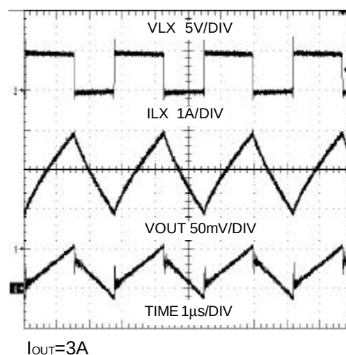
Heavy Load Waveform
