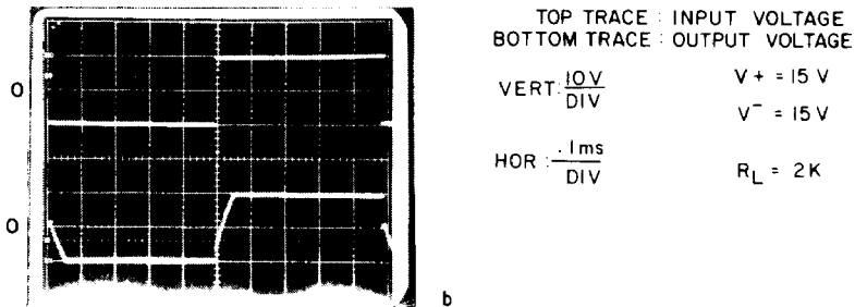
Fig. 18 - Voltage follower (a) test circuit (b) response to 20-V p-p, 1-kHz square-wave input.
