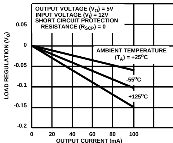
FIGURE 3. LOAD REGULATION WITHOUT CURRENT LIMITING
