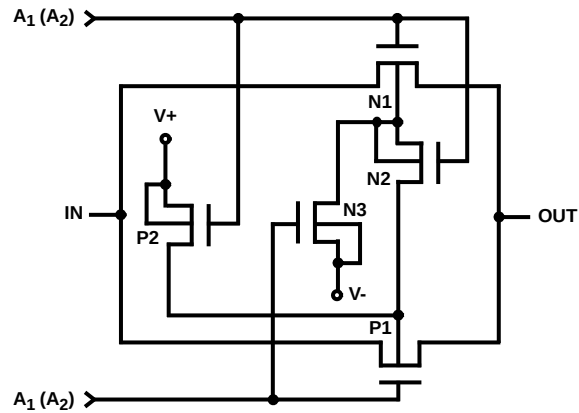
FIGURE 15. SWITCH CELL
