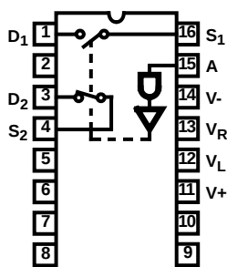
SPDT HI-5042 (50Ω), HI-5050 (25Ω)
