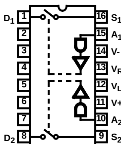
DUAL SPST HI-5048 (25Ω)
