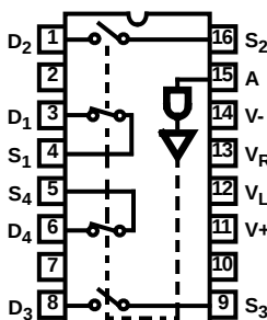
DPDT HI-5046 (50Ω), HI-5046A (25Ω)
