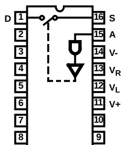
SPST HI-5040 (50Ω)
