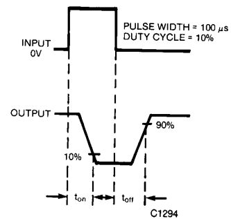
Fig. 11. Switching Time Waveforms
