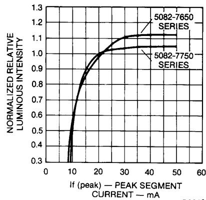
Fig. 3. Relative Efficiency (Average Luminous Intensity Per Unit Intensity Per Unit Current) vs. Peak Current Per Segment
