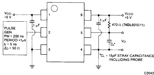
Fig. 15. Switching Time Test Circuit
