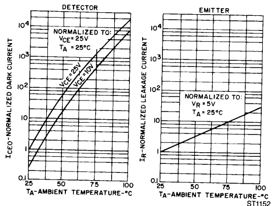
Fig. 4. Leakage Current vs. Temperature
