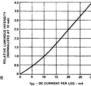
Figure 2. Relative Luminous Intensity vs. Forward Current
