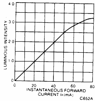
Fig. 2. Luminous Intensity vs. Forward Current
