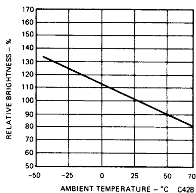
Fig. 2. Relative Luminous Intensity vs. Temperature
