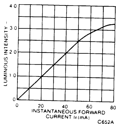
Fig. 2. Luminous Intensity vs. Forward Current
