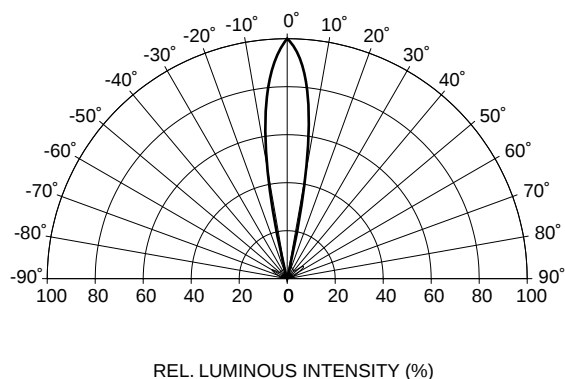
Fig. 4 Radiation Diagram
