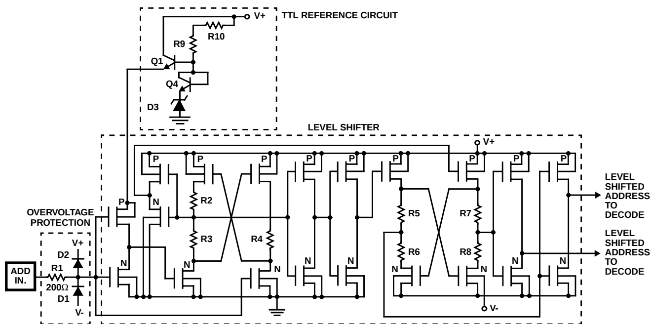
FIGURE 4. ADDRESS INPUT BUFFER AND LEVEL SHIFTER
