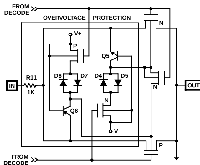
FIGURE 6. MULTIPLEX SWITCH
