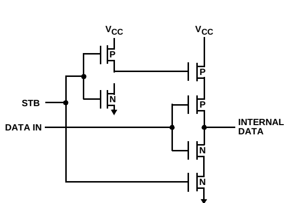
FIGURE 16. 82C82/83H
