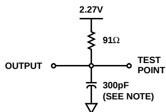
FIGURE 5. TIVOV, TSHOV
