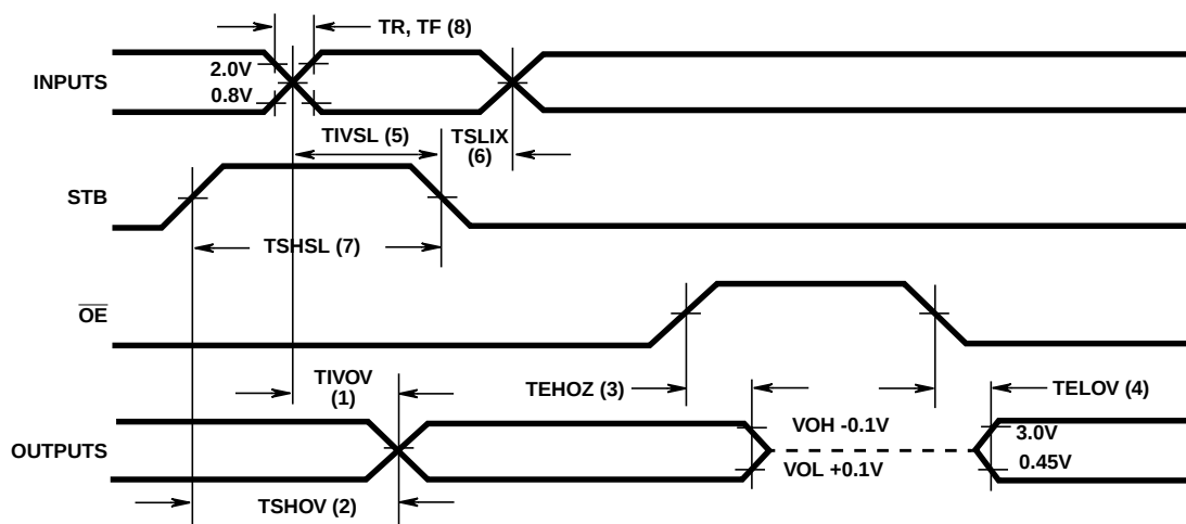
FIGURE 4. TIMING WAVEFORMS
