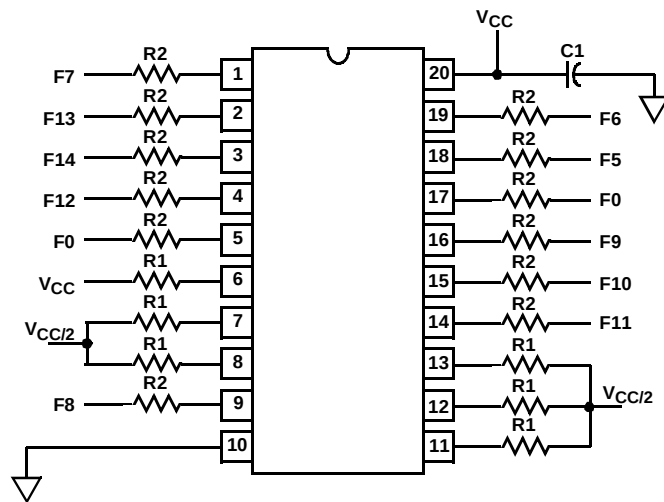
MD82C89 Cerdip
