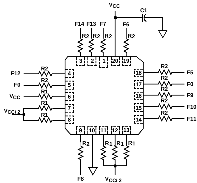
MR82C89 CLCC
