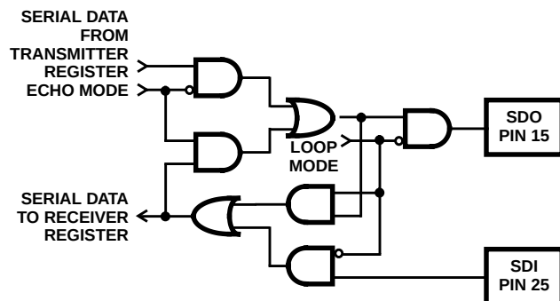
FIGURE 4. LOOP AND ECHO MODE FUNCTIONALITY
