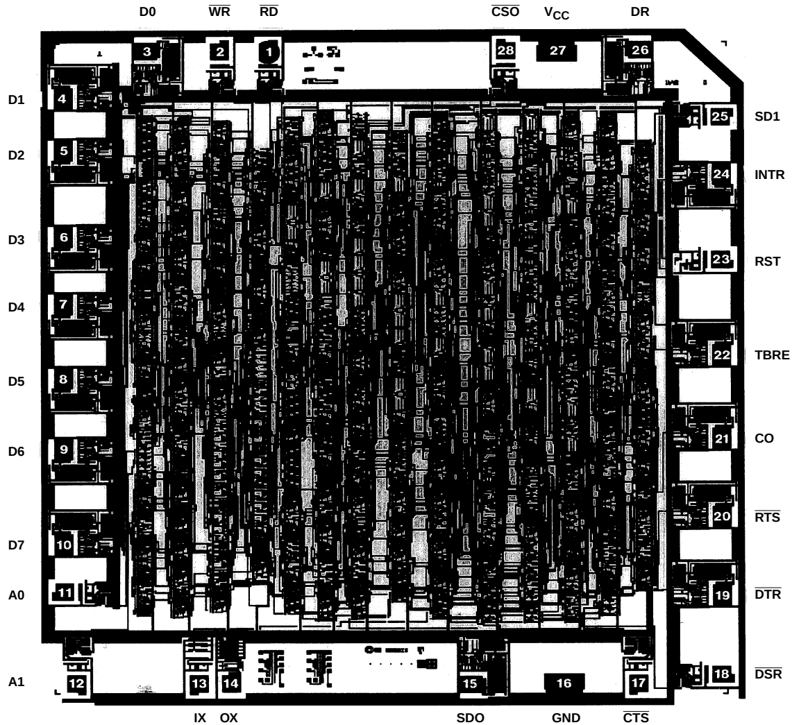
82C52
