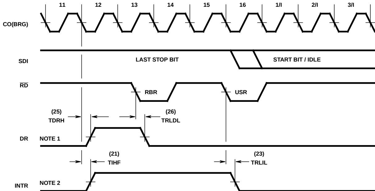
FIGURE 19. RECEIVE TIMING
