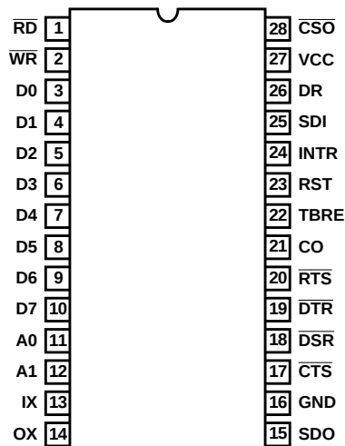
82C52 (PDIP, CERDIP) TOP VIEW
