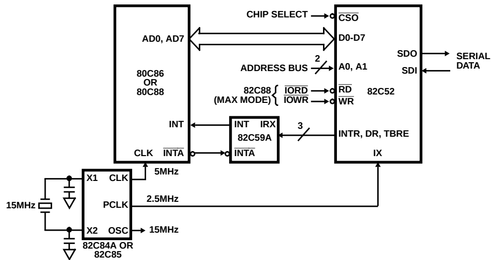
FIGURE 11. 80C86/82C52 INTERFACE
