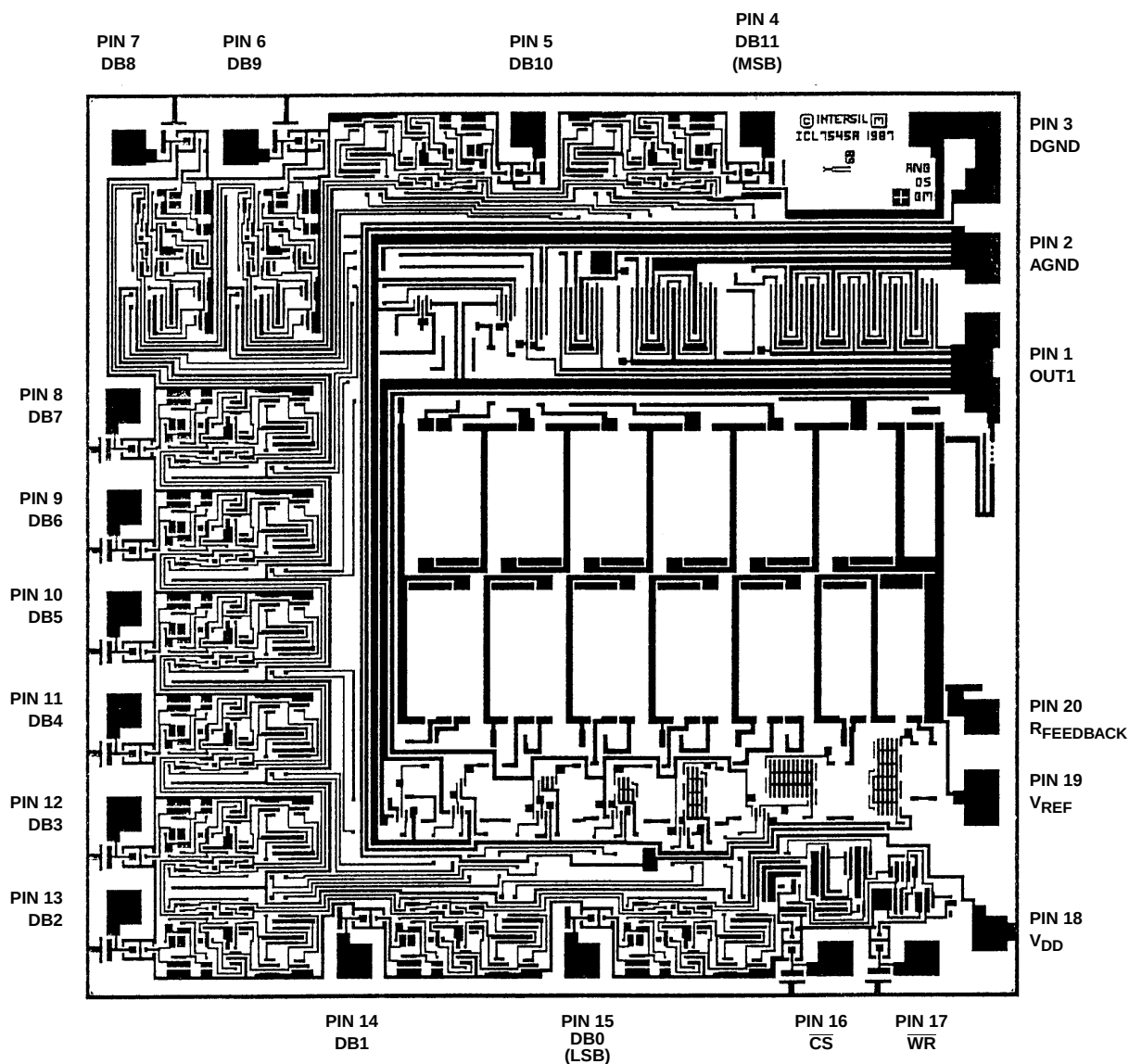
AD7545
