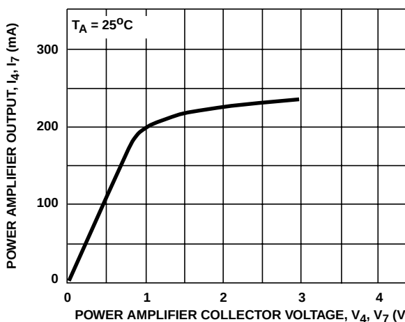
FIGURE 4B. CHARACTERISTIC
