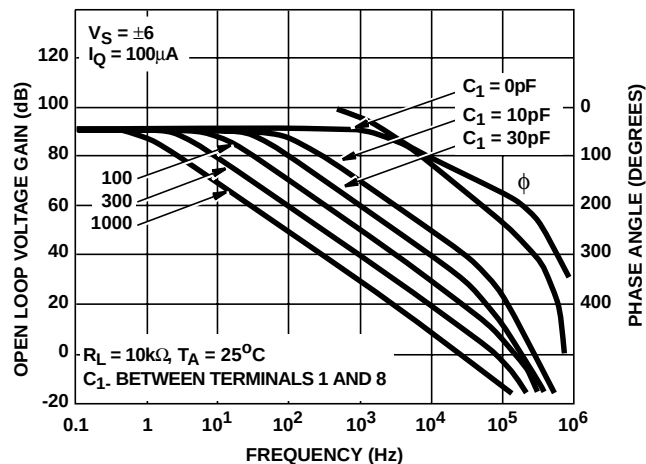
FIGURE 13. OPEN LOOP VOLTAGE GAIN vs FREQUENCY
