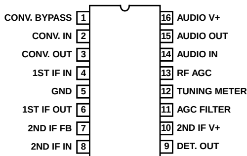
CA3088E (PDIP) TOP VIEW
