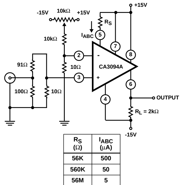
FIGURE 6. OPEN LOOP GAIN vs FREQUENCY TEST CIRCUIT
