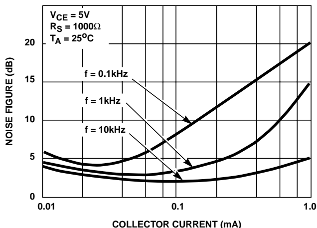
FIGURE 10. NF vs I_C AT R_S = 1k\Omega
