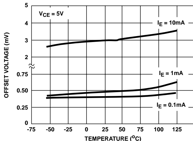
FIGURE 6. V_{IO} vs TEMPERATURE FOR Q_1 AND Q_2
