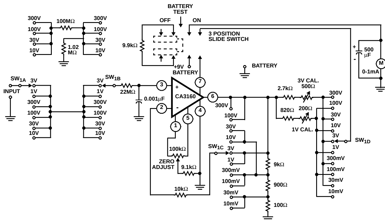
FIGURE 8. HIGH INPUT RESISTANCE DC VOLTMETER
