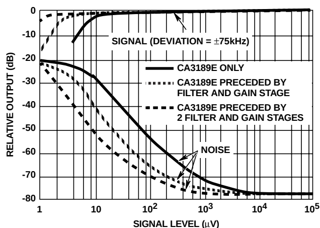
FIGURE 7. TYPICAL LIMITING AND NOISE CHARACTERISTICS
