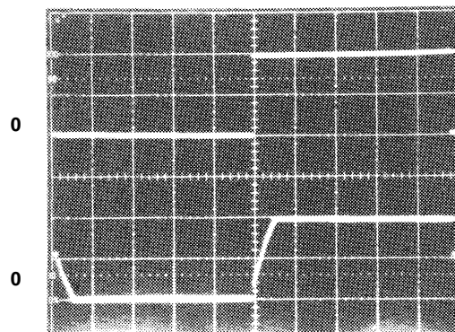
FIGURE 3B. RESPONSE TO 20V P-P , 1kHz SQUARE WAVE INPUT Top Trace: Input Voltage; Bottom Trace: Output Voltage Vertical Scale: 10V/Div.; Horizontal Scale: 0.1ms/Div.
