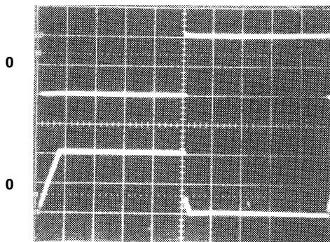
FIGURE 2B. RESPONSE TO 1kHz, 20V P-P SQUARE WAVE Top Trace: Input Voltage, Bottom Trace: Output Voltage Vertical Scale: 10V/Div., Horizontal Scale: 0.1ms/Div.
