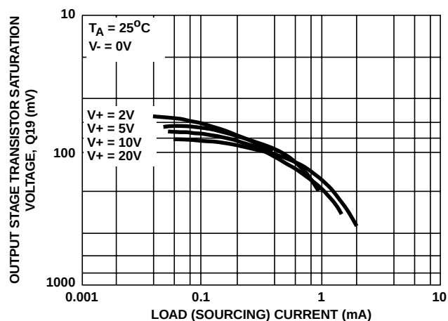
FIGURE 4. OUTPUT VOLTAGE vs LOAD SOURCING CURRENT
