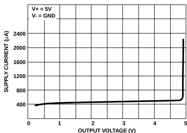
FIGURE 6. SUPPLY CURRENT vs OUTPUT VOLTAGE
