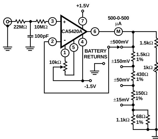
FIGURE 2. HIGH INPUT RESISTANCE VOLTMETER
