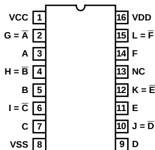
CD4009UBMS TOP VIEW
