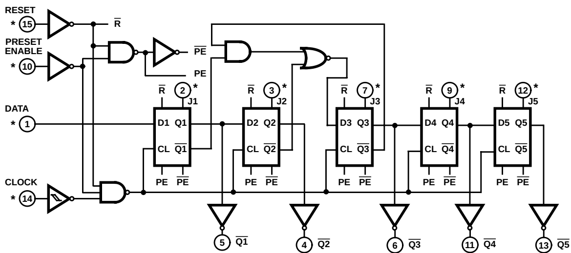
FIGURE 1. LOGIC DIAGRAM
