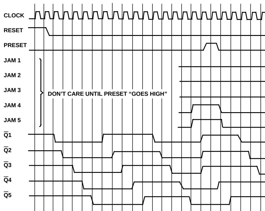
FIGURE 11. TIMING DIAGRAM
