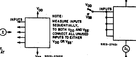
Fig. 20—Input leakage current test circuit.
