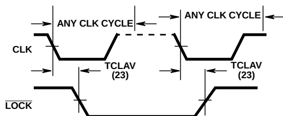
FIGURE 29. BUS LOCK SIGNAL TIMING (MAXIMUM MODE ONLY)
