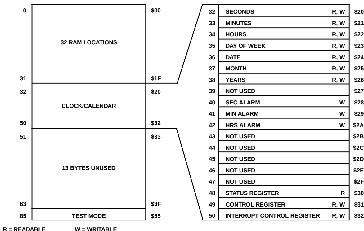
FIGURE 2. ADDRESS MAP
