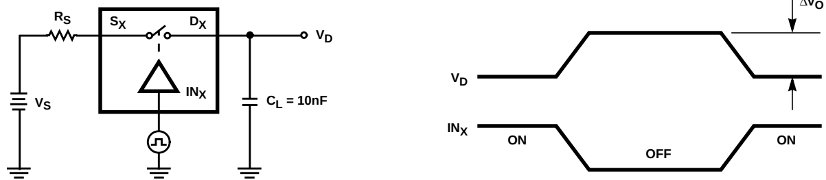
FIGURE 1. CHARGE INJECTION TEST CIRCUIT AND MEASUREMENT POINTS
