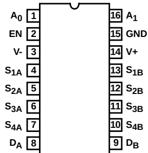
DG409 (PDIP, SOIC)
