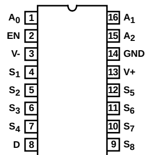
DG408 (PDIP, SOIC)
