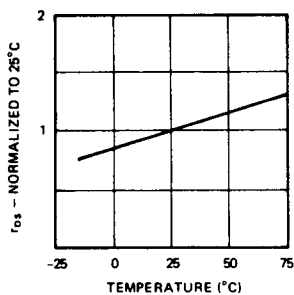
r_{DS(ON)} vs TEMPERATURE (Normalized to 25 ^{\circ}\text{C} Value)
