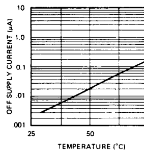
OFF SUPPLY CURRENT vs TEMPERATURE
