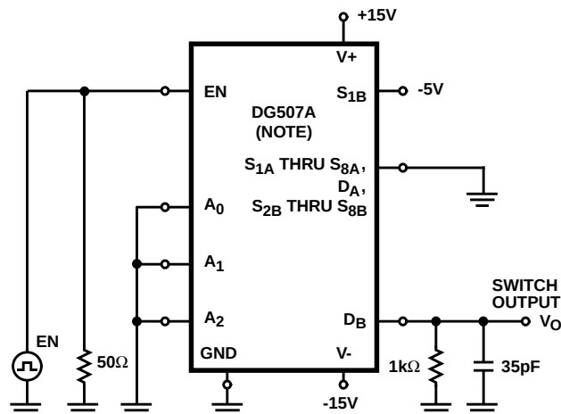
FIGURE 1. SWITCHING TIME
