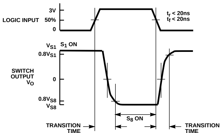
FIGURE 1C. MEASUREMENT POINTS
