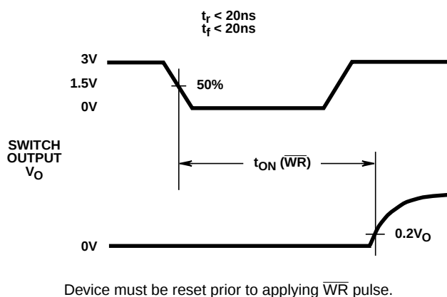
FIGURE 6A. WRITE t_{ON} SWITCHING TIME WAVEFORMS
