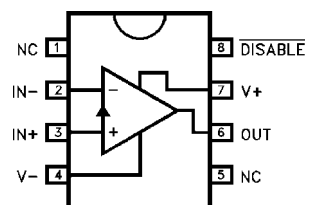
EL2120 (8-PIN SO) TOP VIEW
