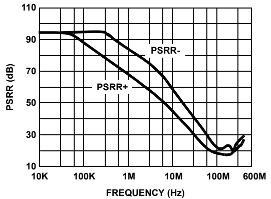
FIGURE 30. PSRR
