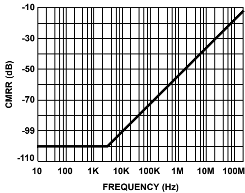
FIGURE 29. CMRR
