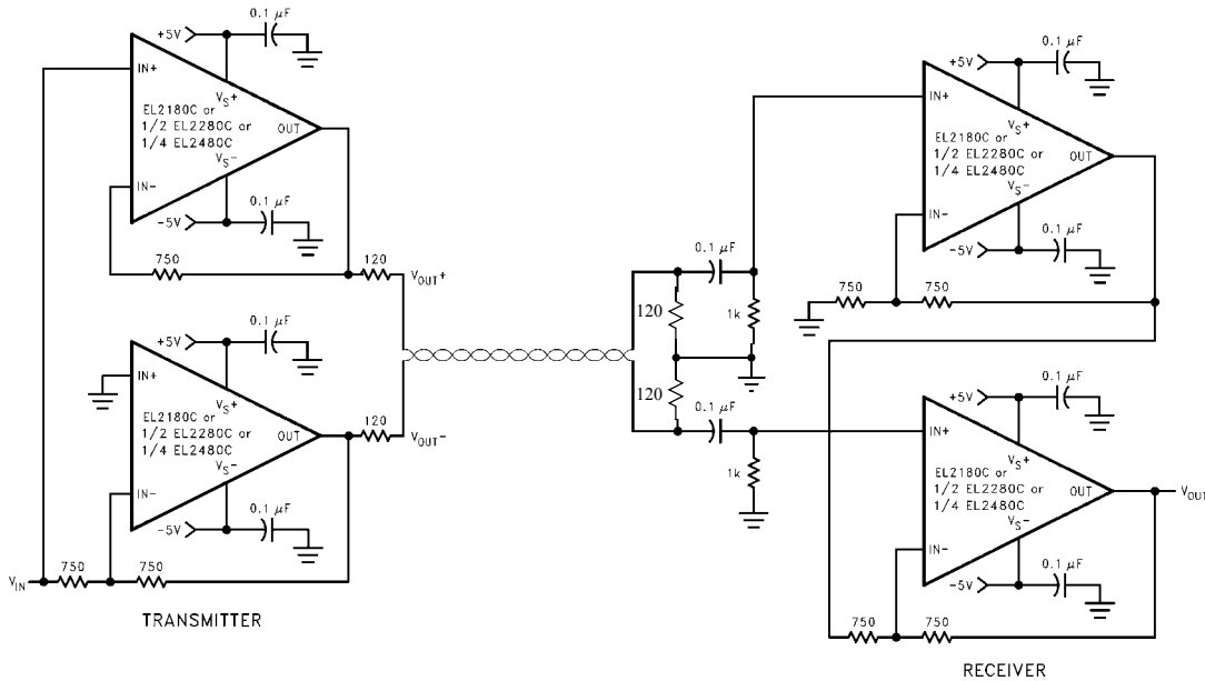
DIFFERENTIAL LINE-DRIVER/RECEIVER
