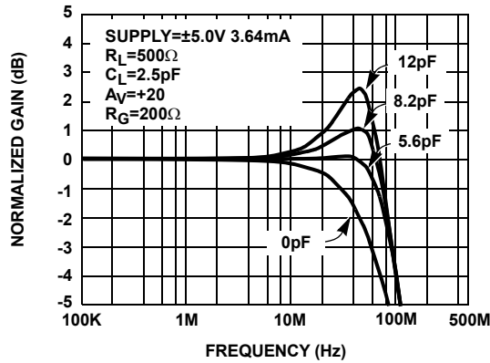
FIGURE 1. GAIN vs FREQUENCY FOR VARIOUS C_{IN}
