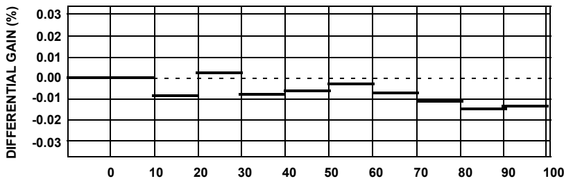
FIGURE 26. DIFFERENTIAL GAIN (%)
