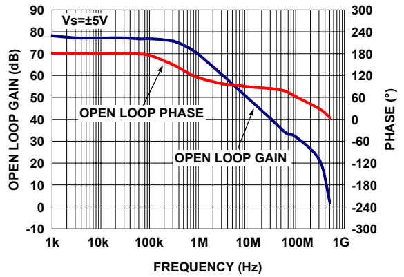
FIGURE 16. OPEN LOOP GAIN & PHASE vs FREQUENCY
