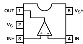
EL5191 (5-PIN SOT-23) TOP VIEW
