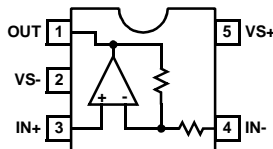
EL5197 (5-PIN SOT-23) TOP VIEW
