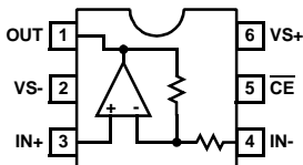
EL5197A (6-PIN SOT-23) TOP VIEW
