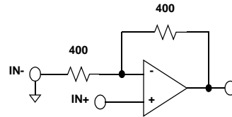
FIGURE 1. A_V = +2
