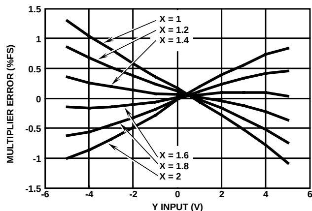
MULTIPLIER ERROR
