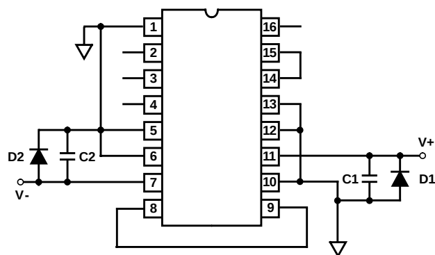
HA-2546/883 CERDIP
