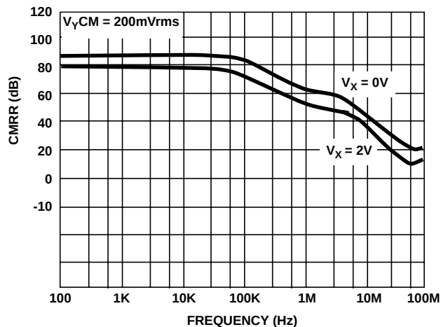
V_Y CMRR vs FREQUENCY
