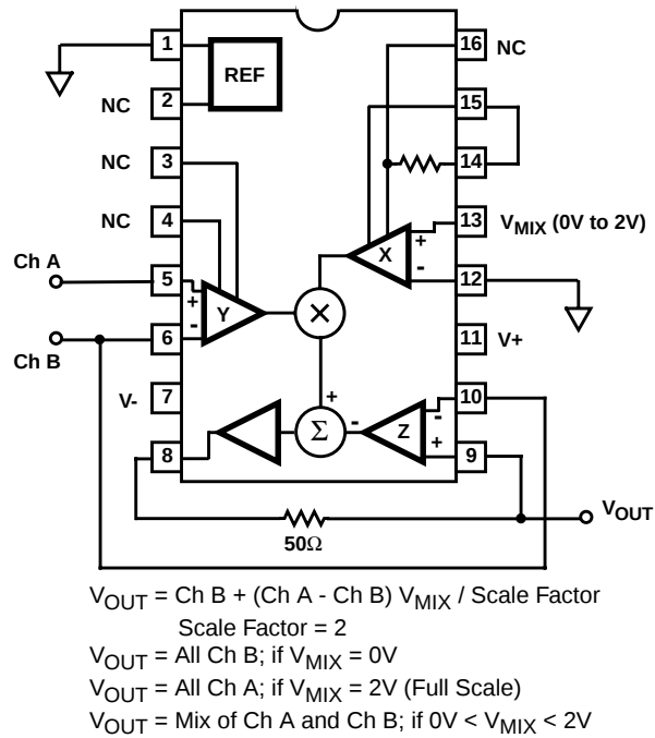
FIGURE 6. VIDEO FADER
