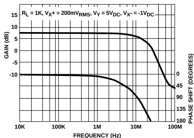
FIGURE 8. V_X GAIN AND PHASE vs FREQUENCY
