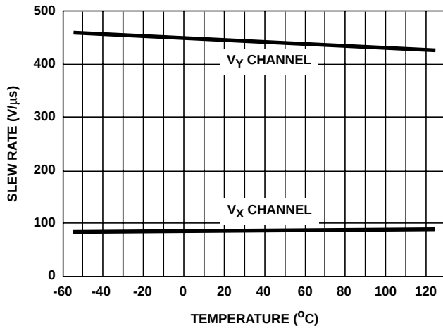
FIGURE 33. SLEW RATE vs TEMPERATURE
